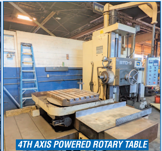
TOSHIBA SHIBAURA LTD-9 BORING MILL
