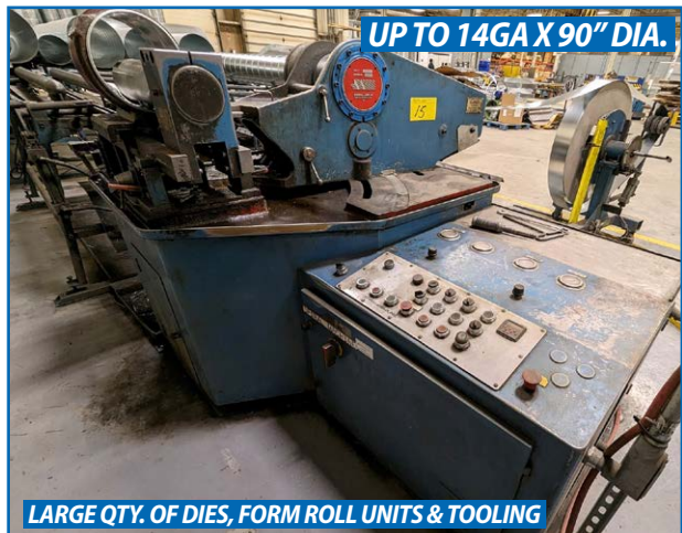
SPIRAL-HELIX 200H SPIRAL TUBE FORMER DUCT LINE
